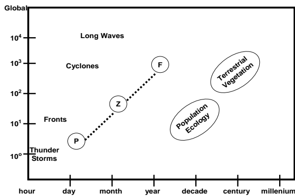
Figure 1.2. Comparison of time-space scales: Physical atmospheric processes (thunderstorms to long waves), physical mixing processes in the oceans (dashed line), and marine and terrestrial ecosystems.
