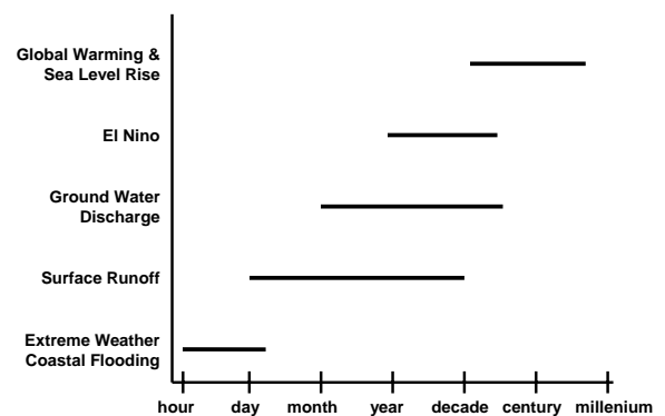
Figure 1.3. Time Scales of Major, Cross-boundary External Forcings in the Coastal Zone: Given the range of time-space scales that must be captured, both remote (satellite, aircraft, ground-based) and in situ sensing will be needed.
