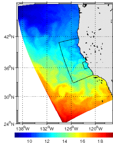
Figure 3.1. Nested regional ocean model for northeastern Pacific (15/5/1.5km resolution)
